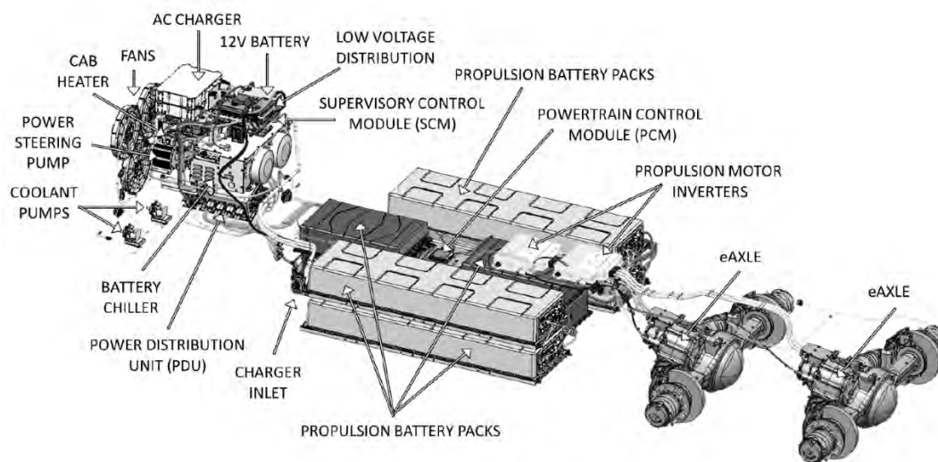
Vehicle Layout
