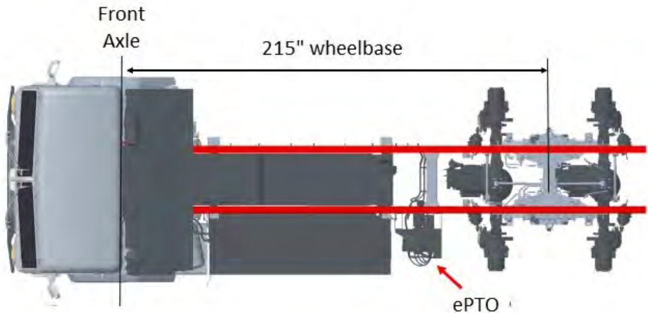
FIGURE 7-1. Model 520 BEV 215" Wheelbase with ePTO
