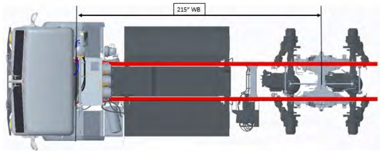
FIGURE 3-3a. 520 BEV 215" Wheelbase
