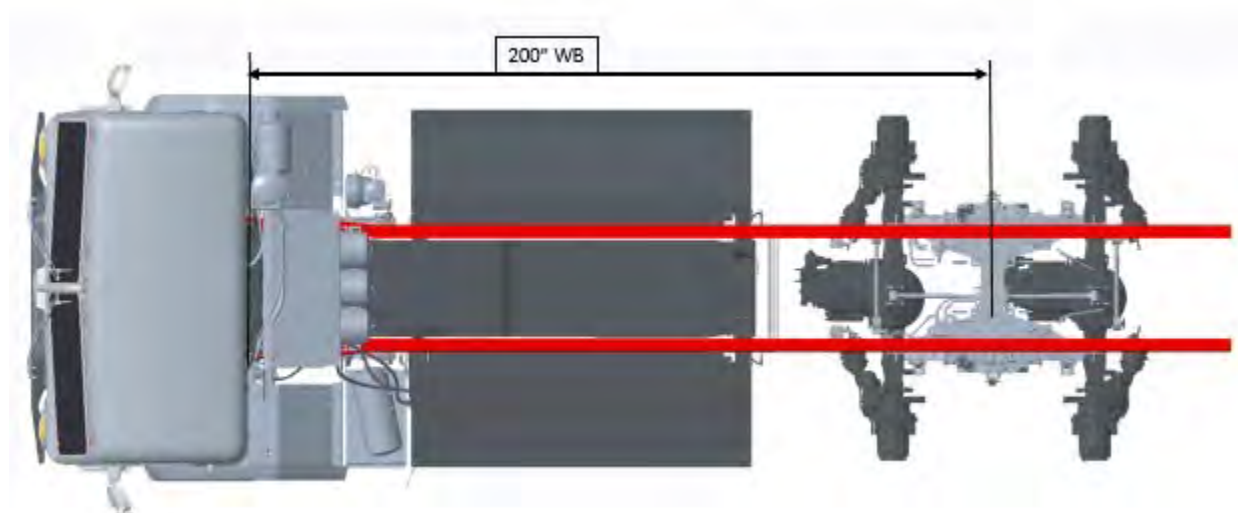
FIGURE 3-3b. 520 BEV 200" Wheelbase
