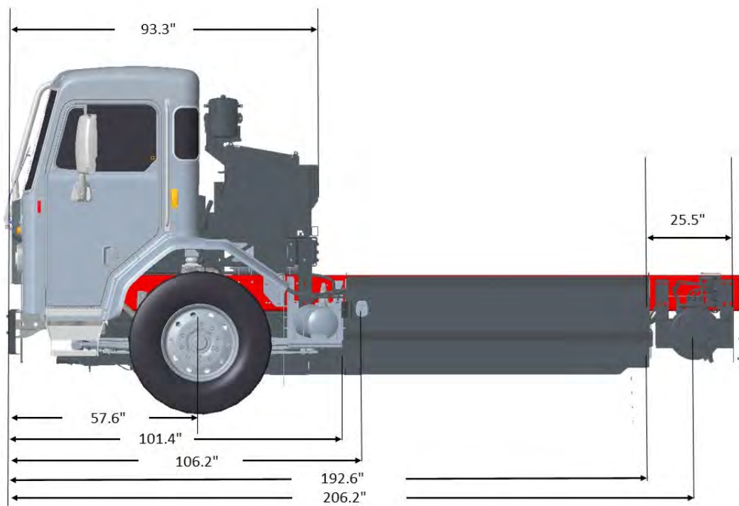
FIGURE 3-2b. 520 BEV Dimensions (Side Loader Configuration)
