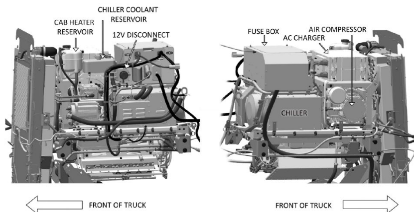
Additional Components on the PCAS
