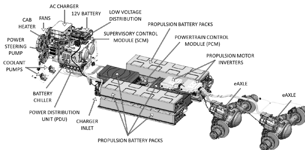
Vehicle Layout
