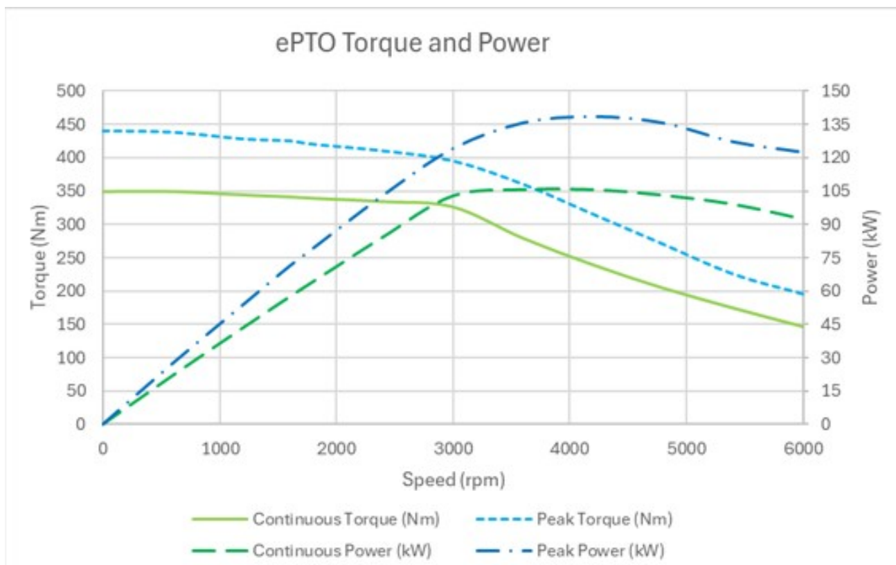
FIGURE 7-6. ePTO Torque and Power Chart
