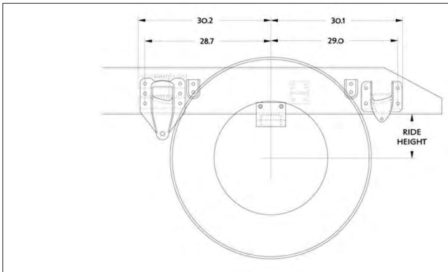
FIGURE 3-5. Reycos 79KB Frame Drilling (Dimensions In Inches)
